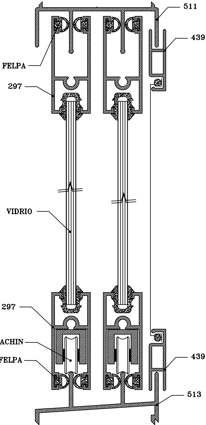
CORTE VERTICAL
