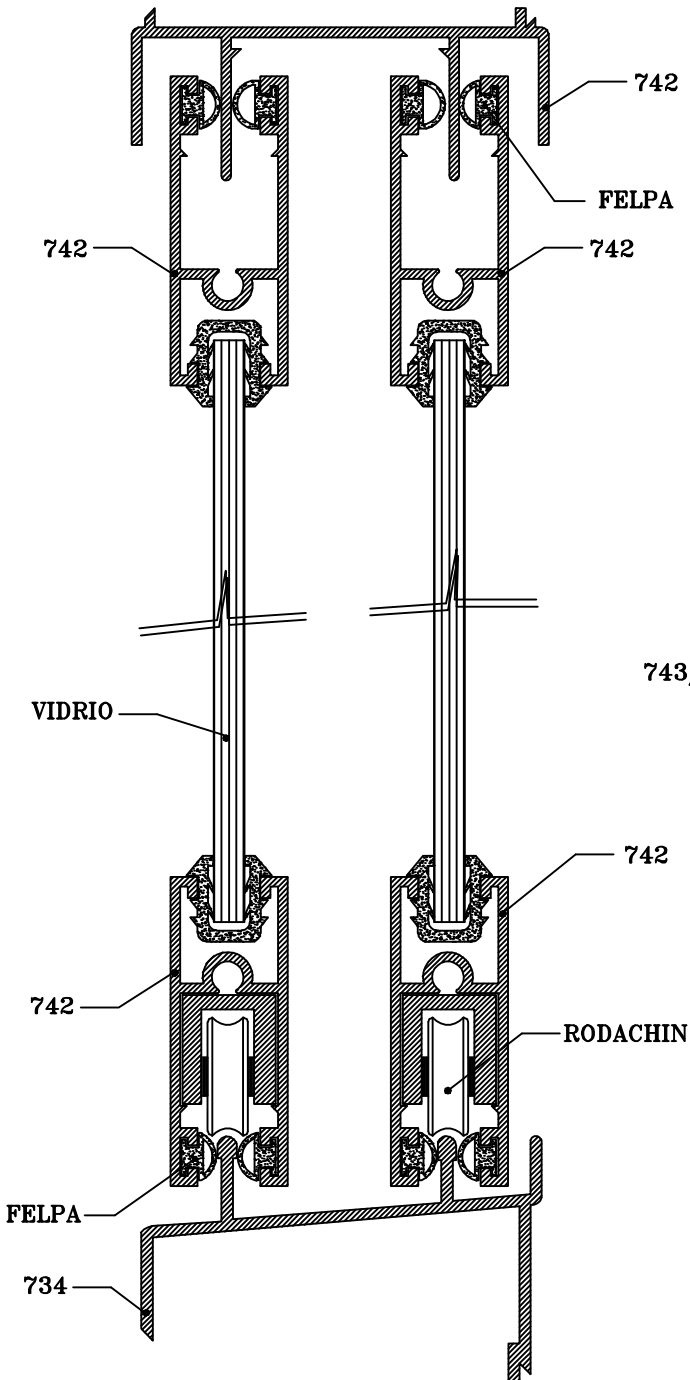
CORTE VERTICAL
