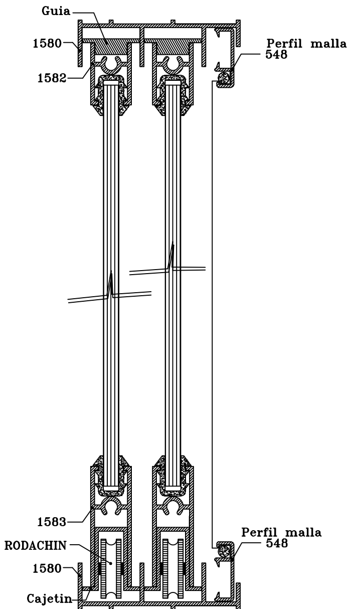
CORTE VERTICAL
